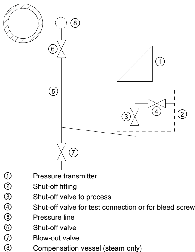
Figure 5-1 Measuring steam
